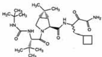
Formula Ia;
