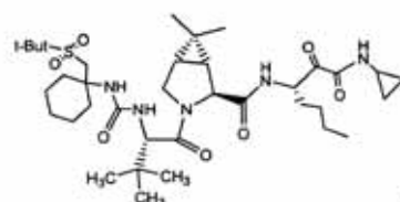
Formula IIb;
