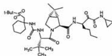
Formula IIc
