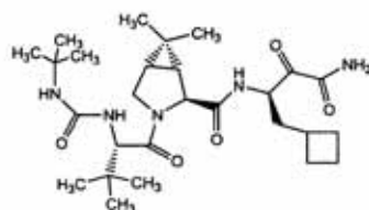
Formula Ic;
