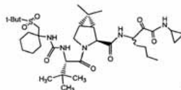
Formula IIa;
