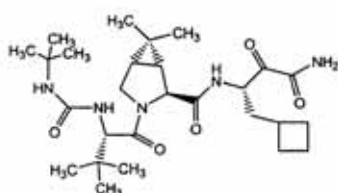
Formula Ib;
