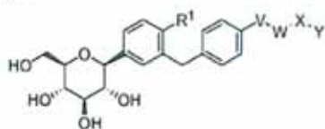
Formula IA:
